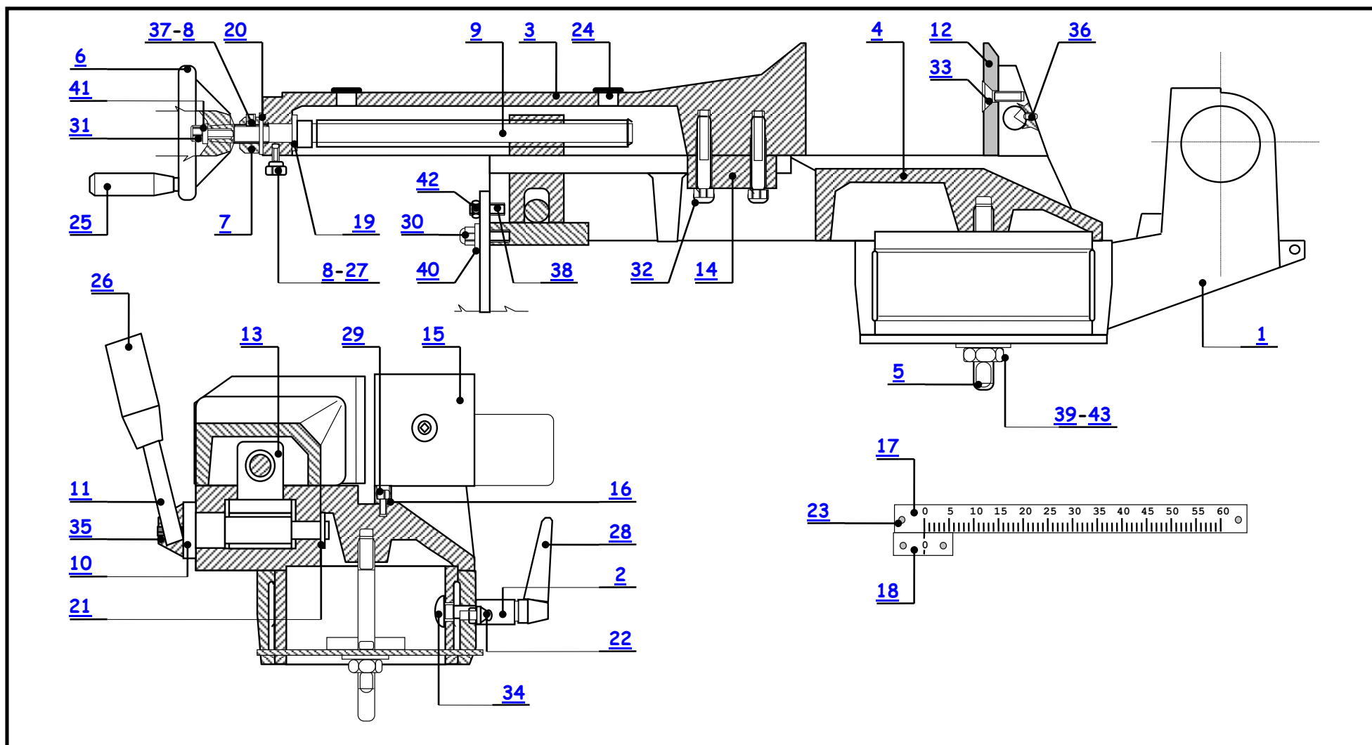
ENSEMBLE ETAU MANUEL
