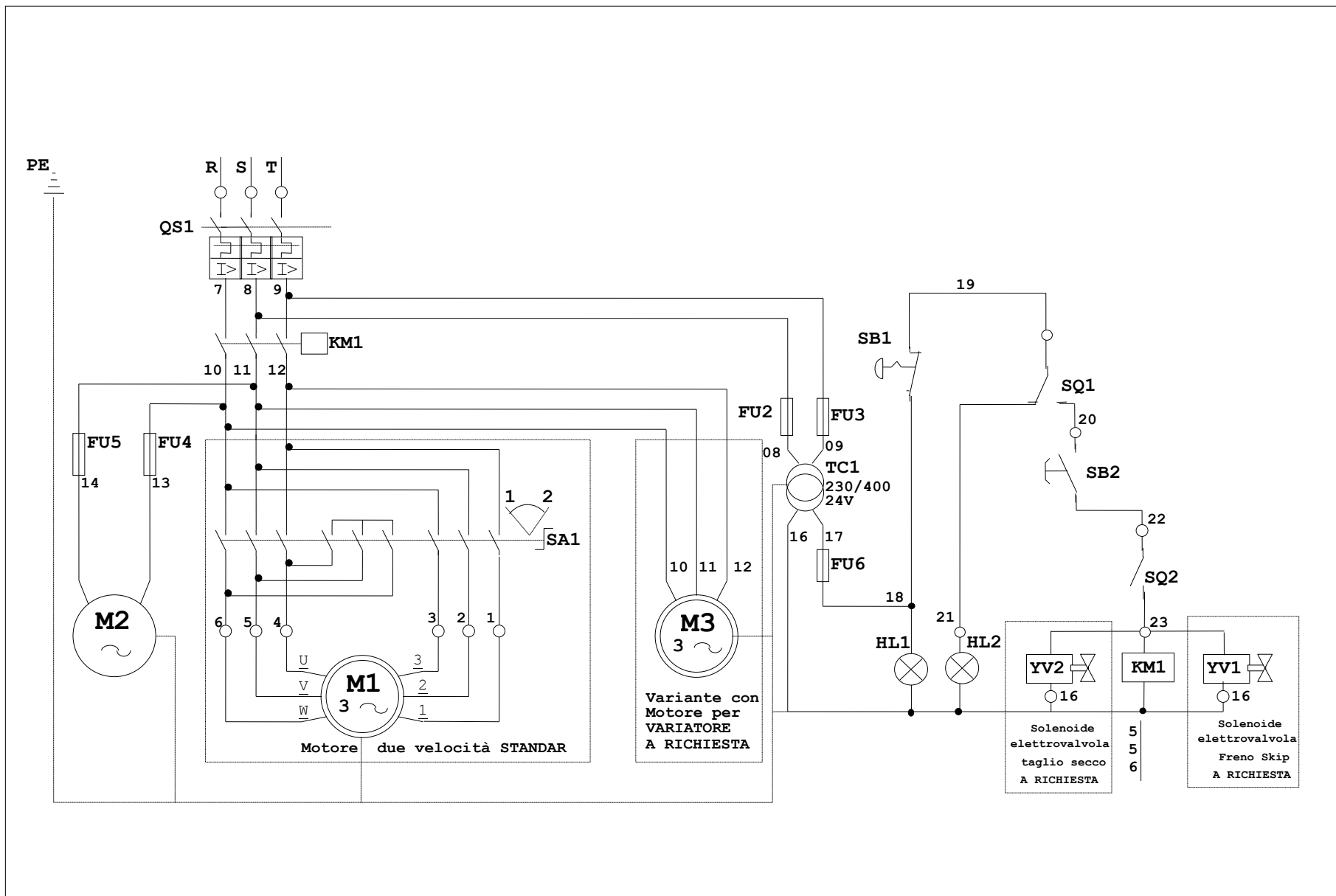
SCHEMA ELECTRIQUE
