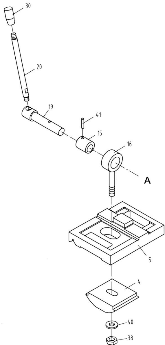
Tailstock Assembly II
