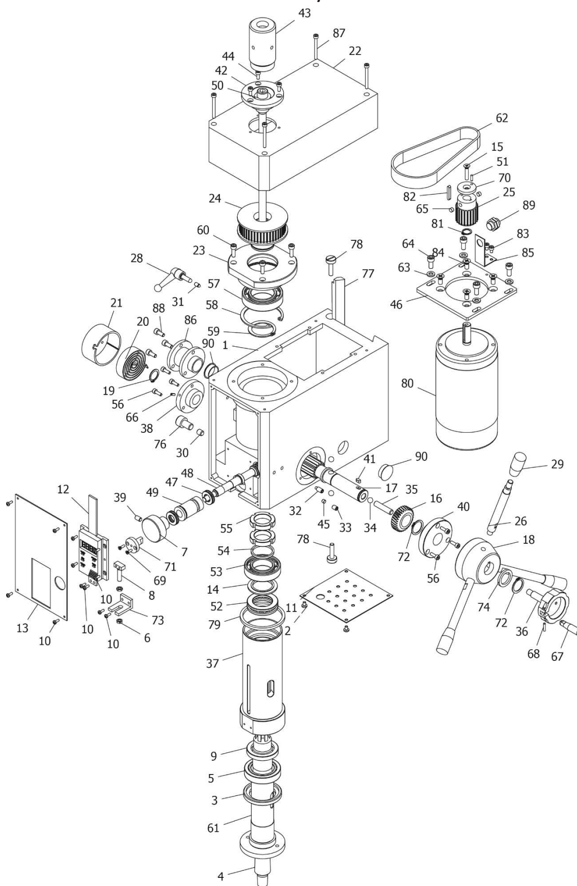
PBM-1839V Assembly Breakdown -1
