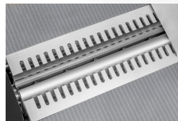
Standard 3 cutter head 310x25x3
